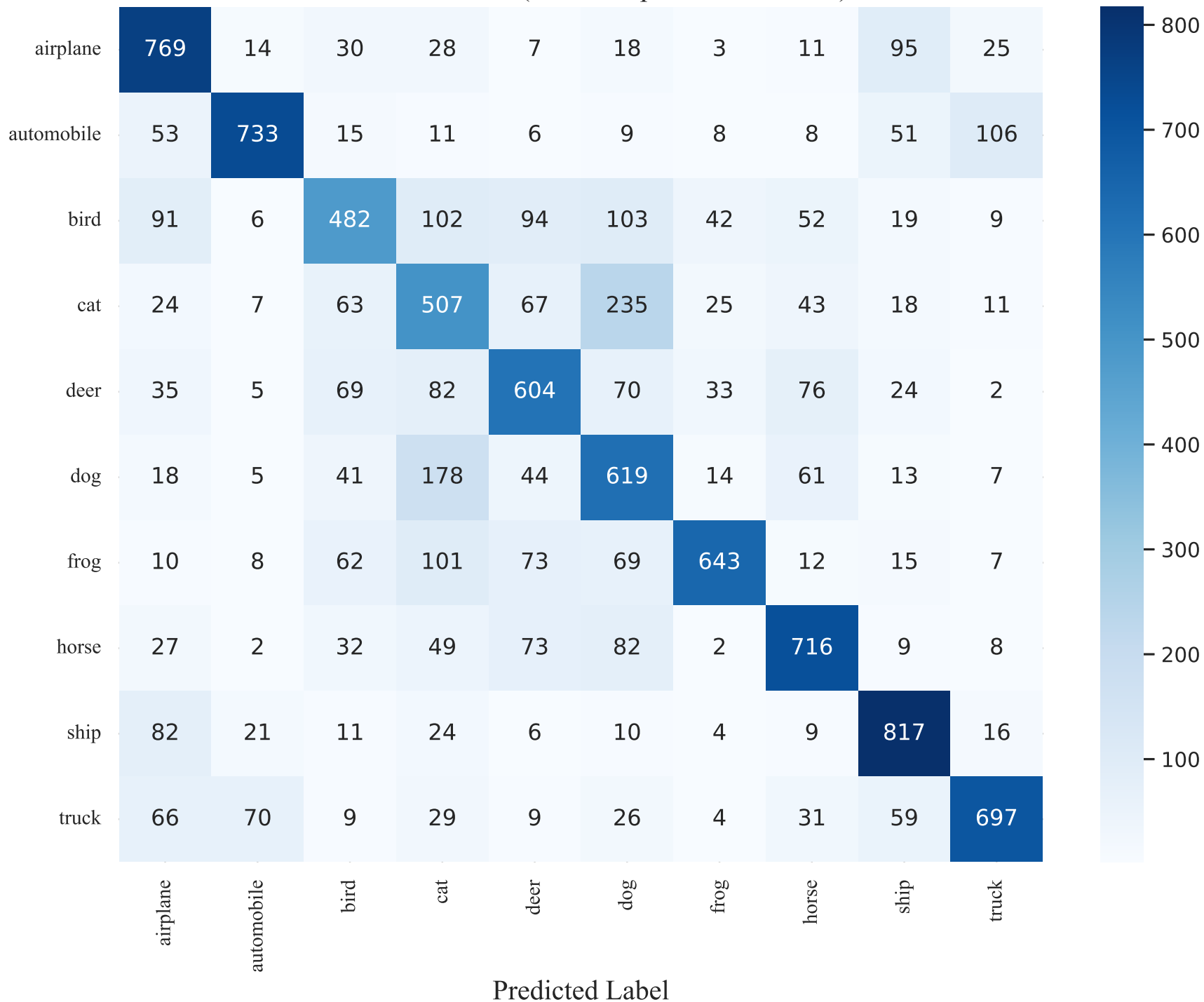
Confusion Matrix (Manual-Specification CNN)
